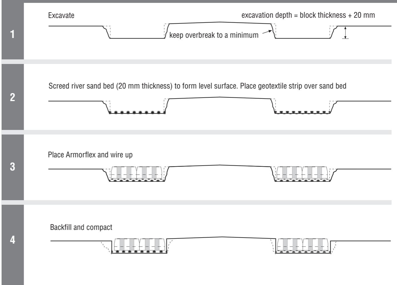
Strip roads excavation procedure
